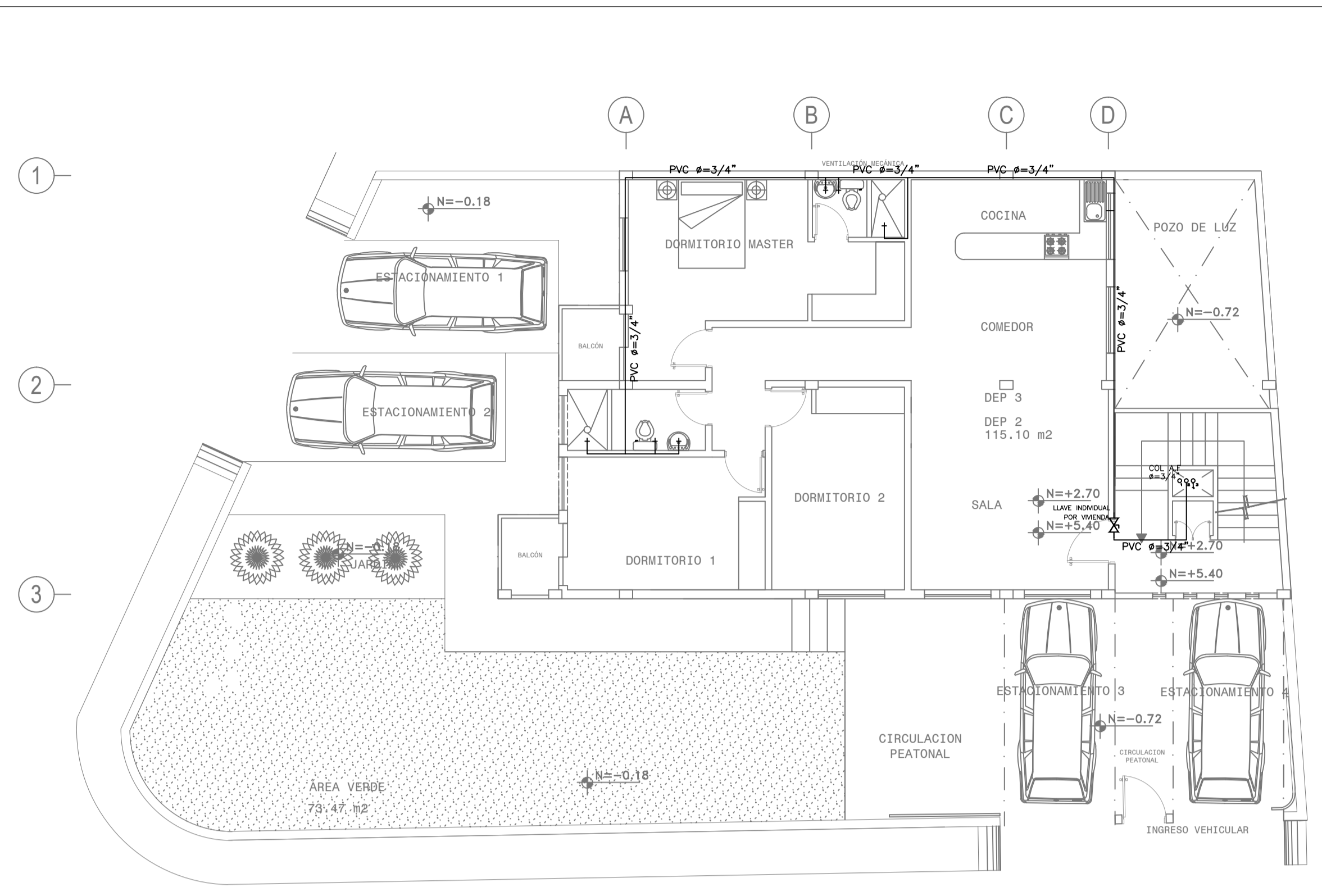
PLANTA ALTA N+2.70 y N+5.40 ESCALA-----1:100
