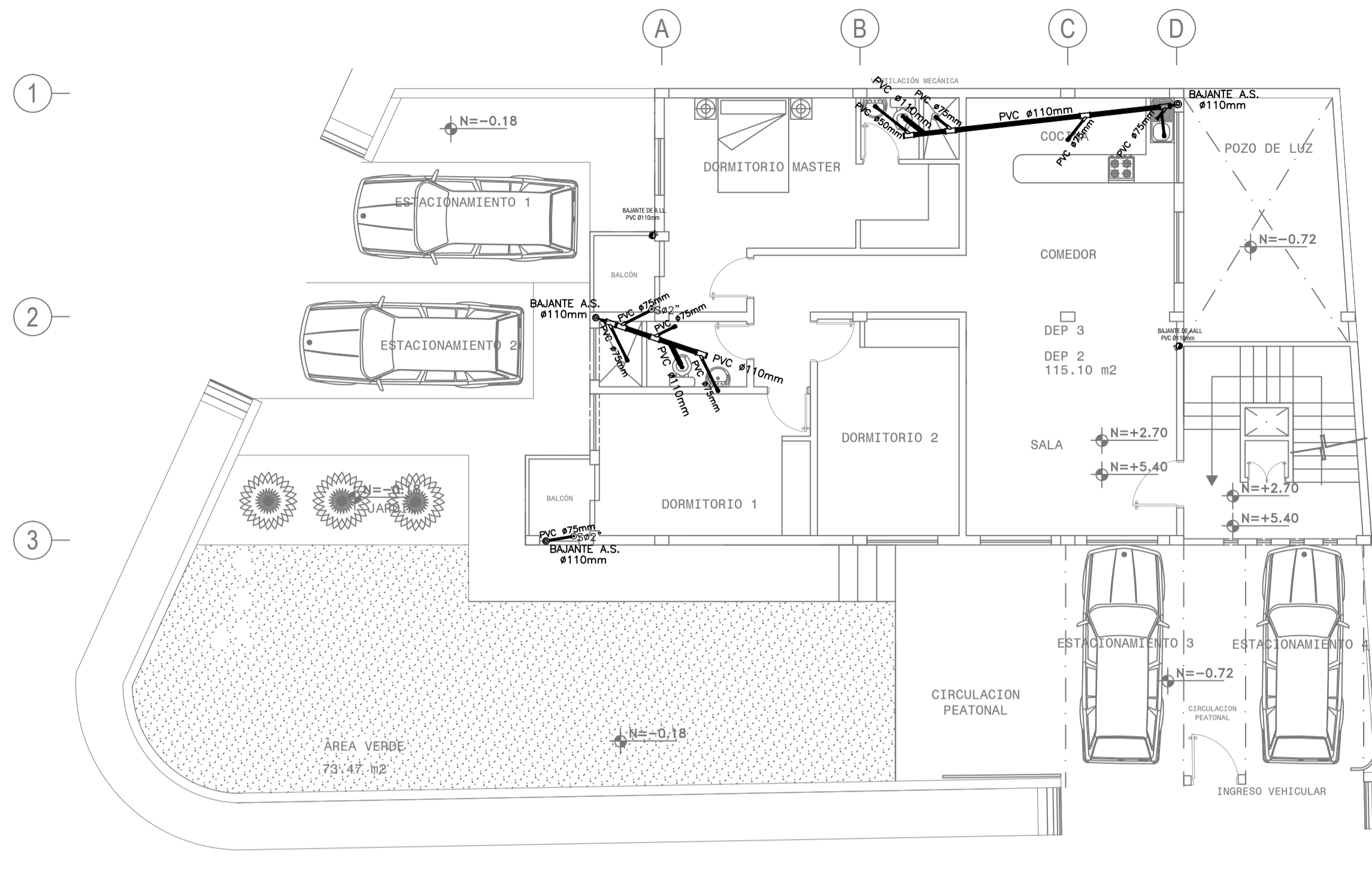
PLANTA ALTA N+2.70 y N+5.40 ESCALA-----1:100
